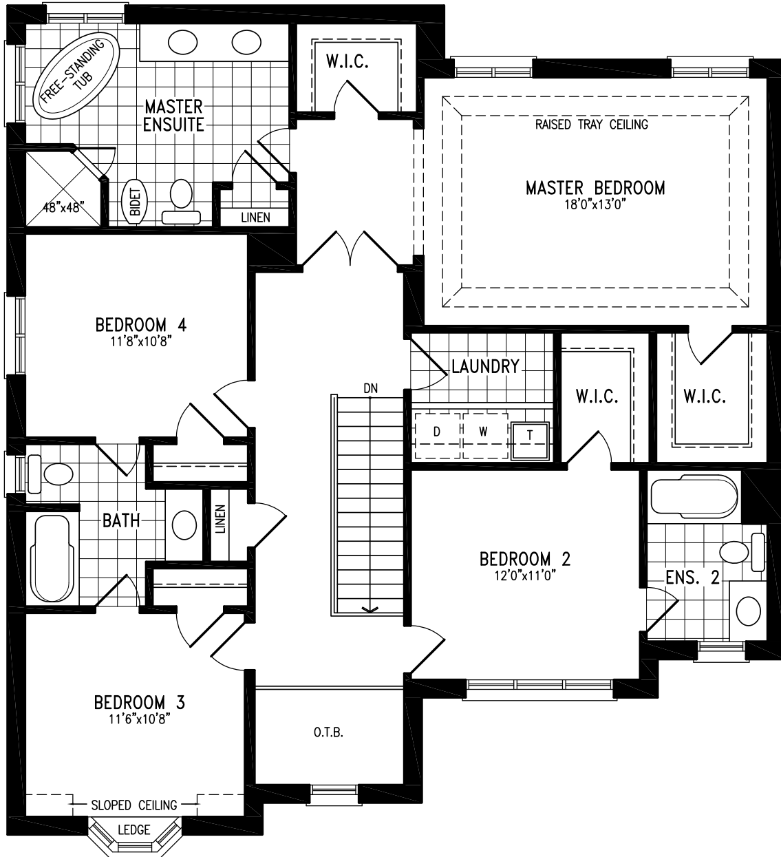
Elevation A SECOND FLOOR
