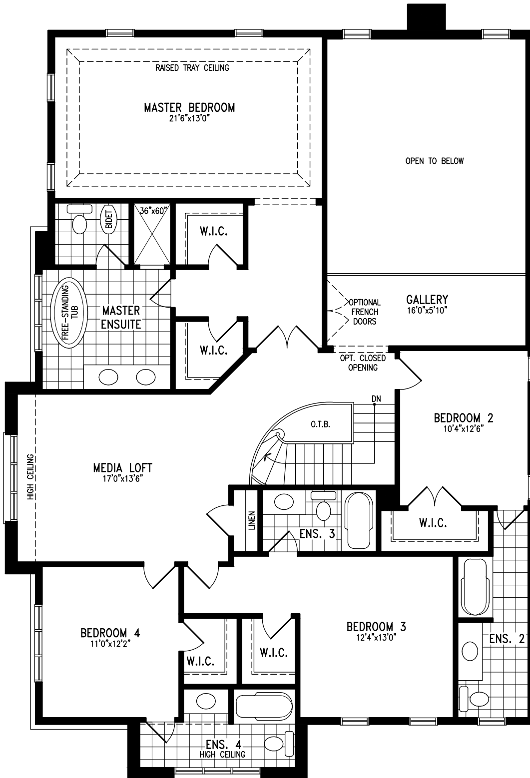
Elevation B SECOND FLOOR
