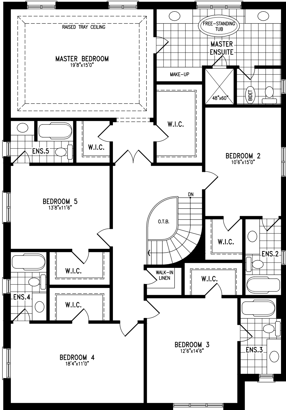
☆ ARCHITECT'S PREMIUM OPTION Elevation A SECOND FLOOR with 5 bedrooms
