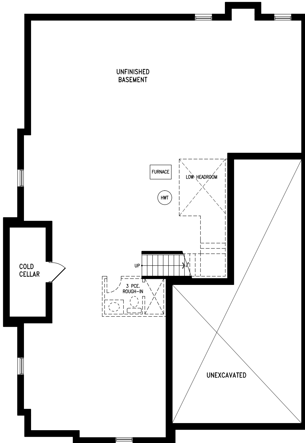
Elevation A BASEMENT
