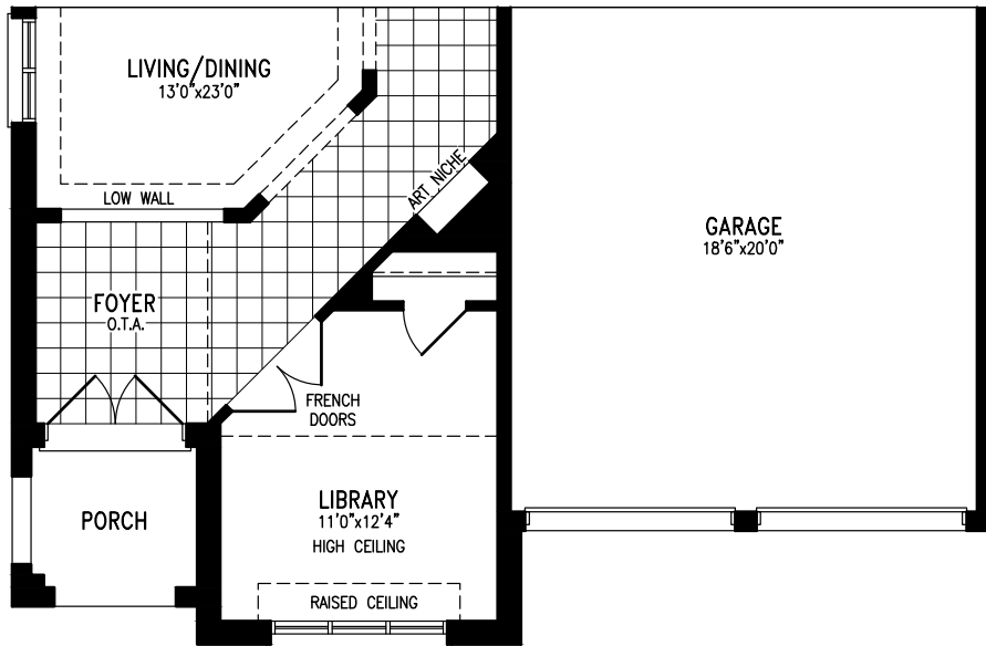
Elevation B GROUND FLOOR
