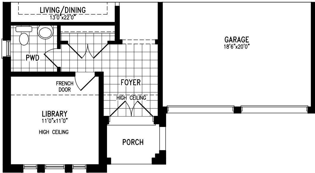
Elevation B GROUND FLOOR
