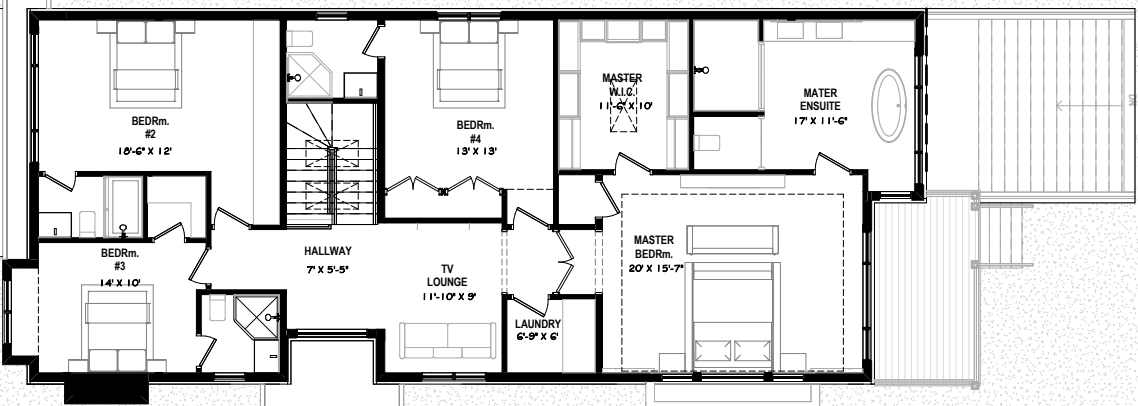
Second Floor
