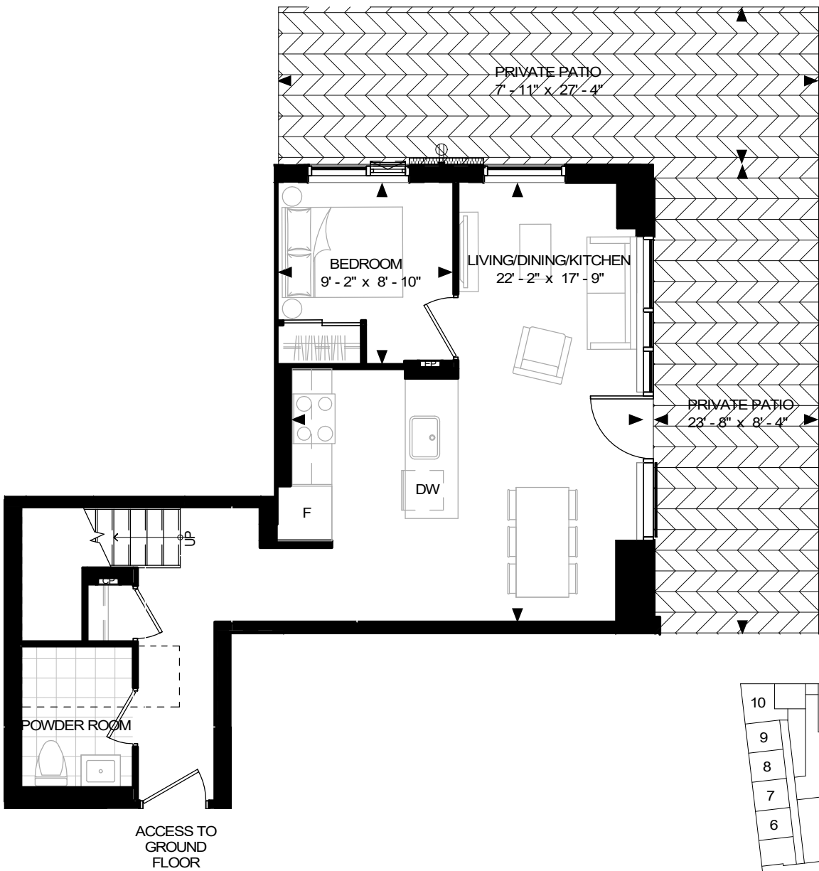
GROUND FLOOR
