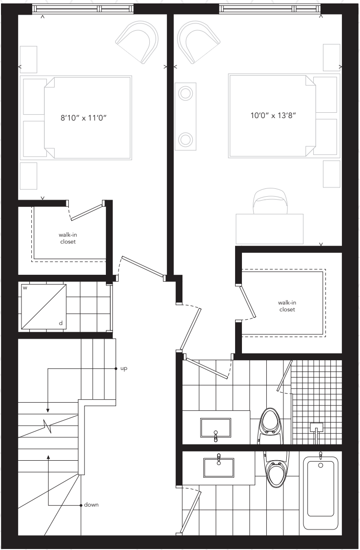
Second Floor
