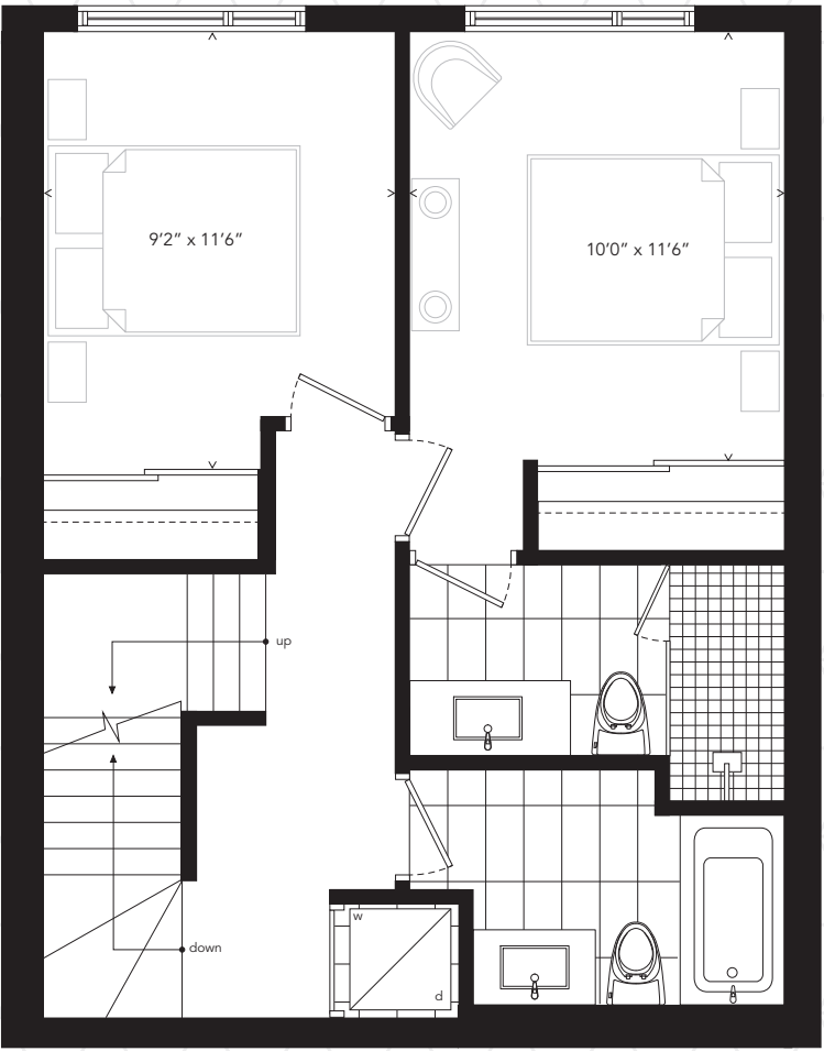
Second Floor
