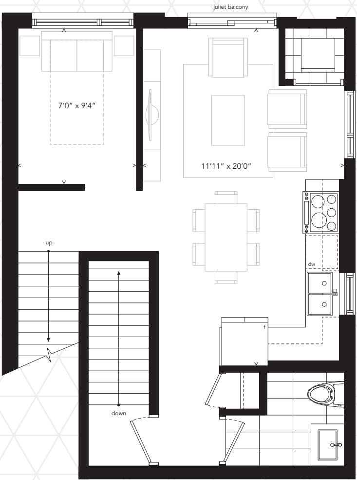
Main Floor
