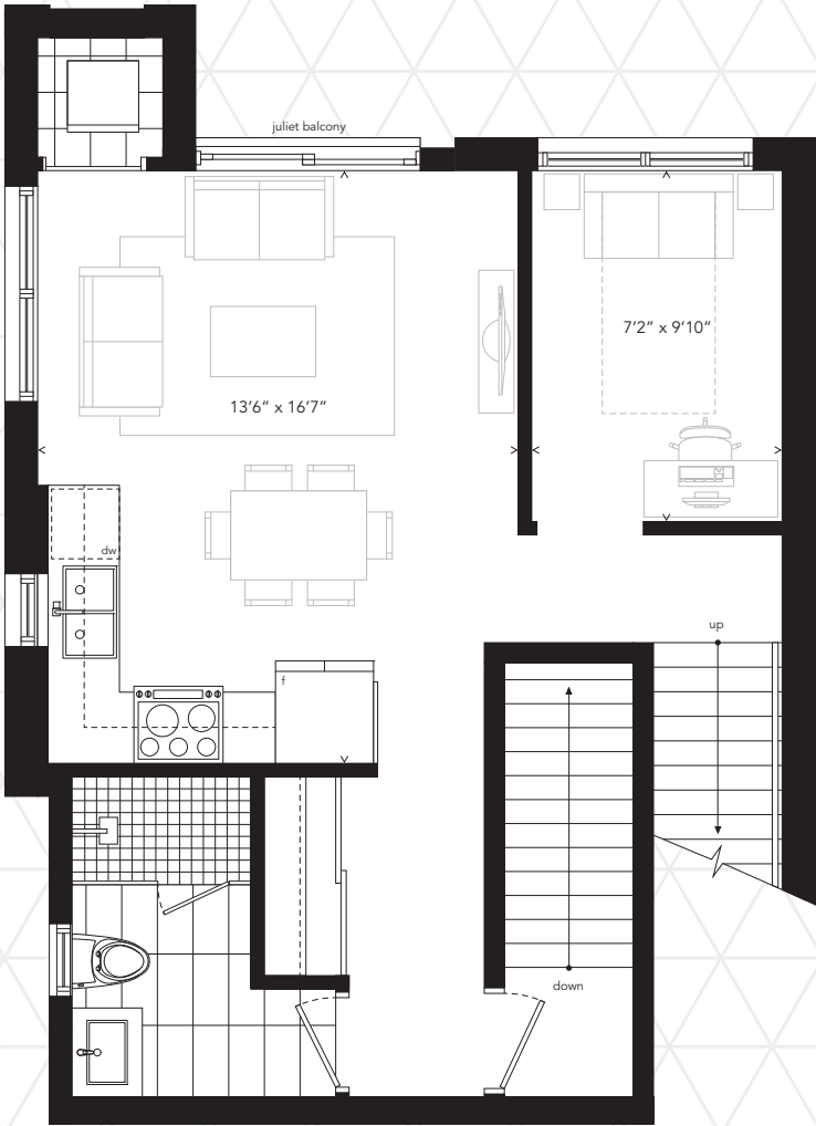
Main Floor
