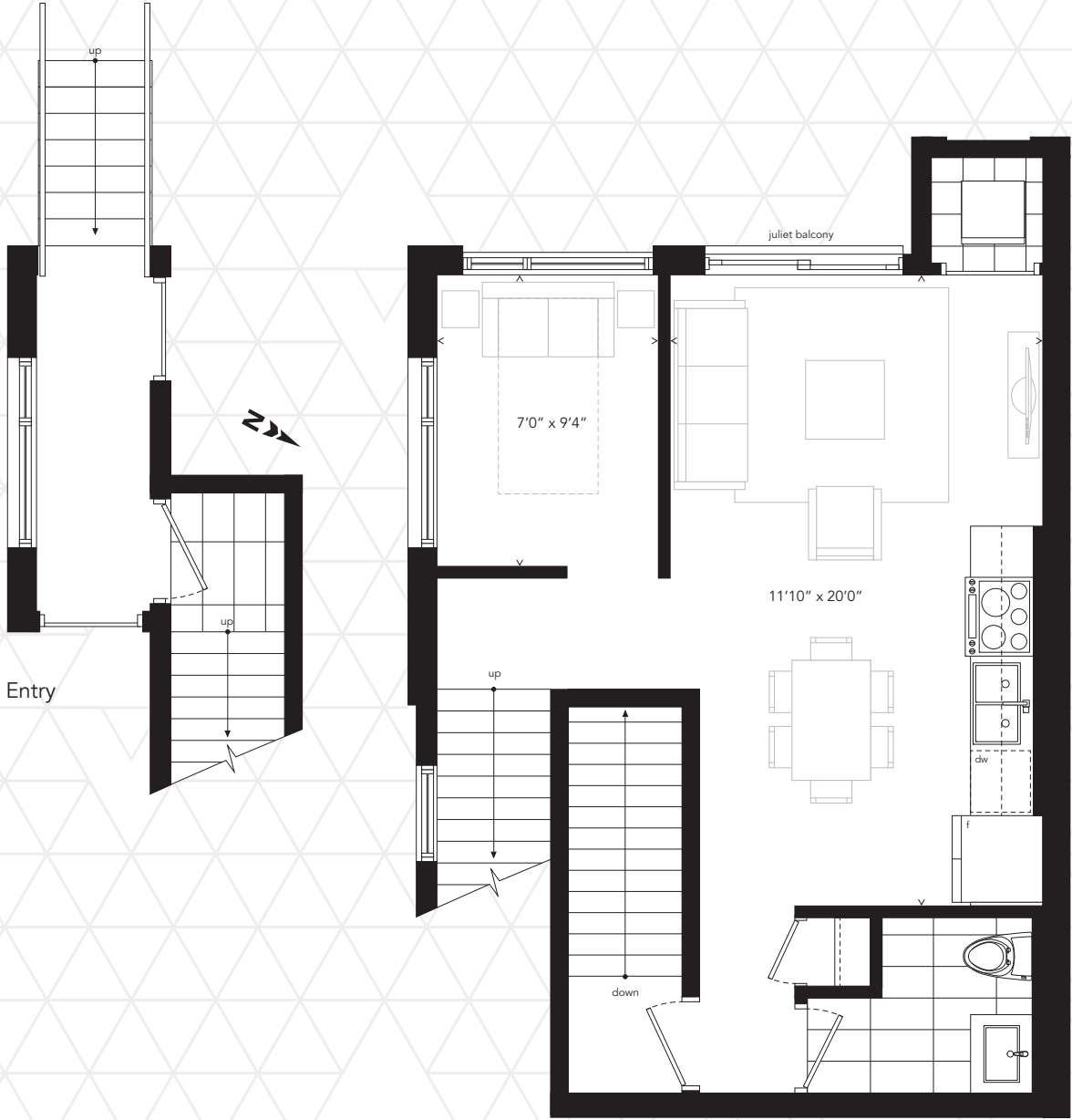
Main Floor
