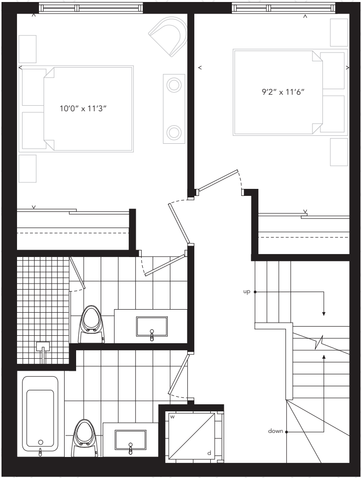
Second Floor
