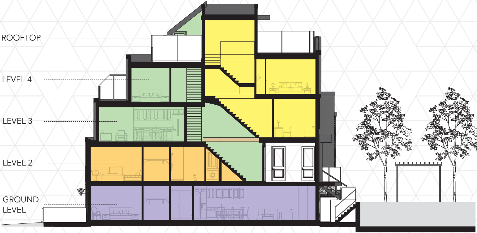
CROSS SECTION
