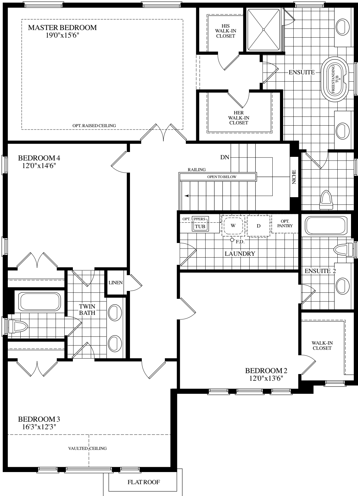
UPPER LEVEL (4 BEDROOM) ELEV. A FOR OPT. MAIN LEVEL
