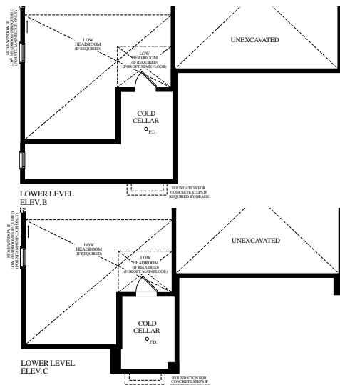
LOWER LEVEL ELEV. C
