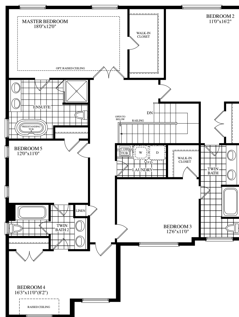
OPT. 5 BEDROOM UPPER LEVEL ELEV. A
