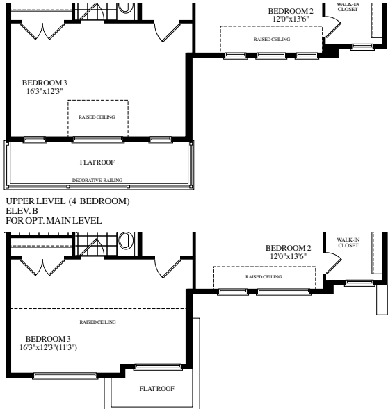
UPPER LEVEL (4 BEDROOM) ELEV. B FOR OPT. MAIN LEVEL
