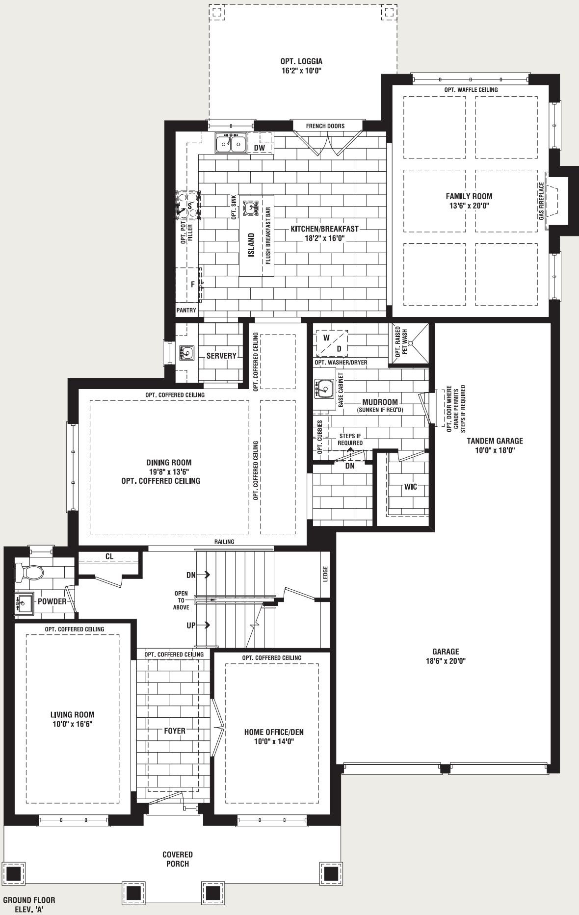
GROUND FLOOR ELEV. 'A'
