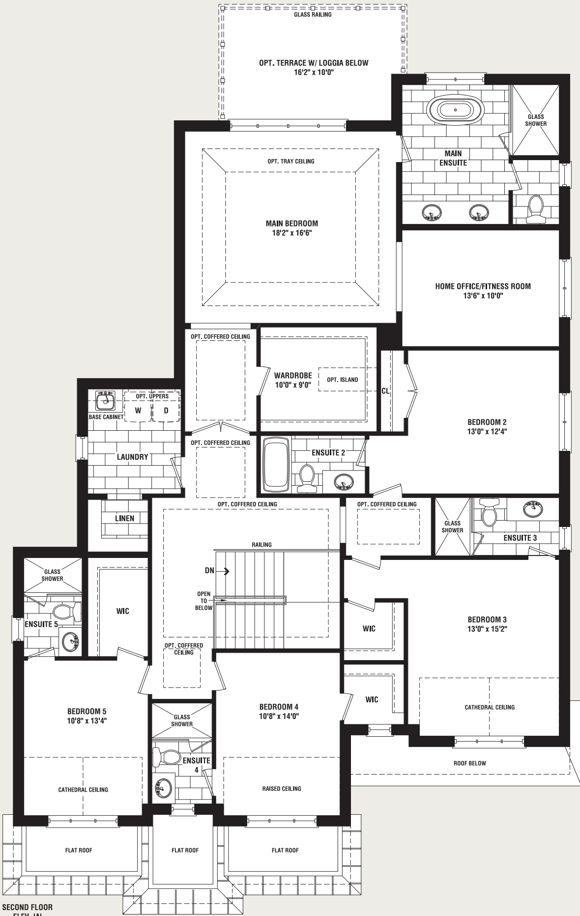
SECOND FLOOR ELEV. 'A'
