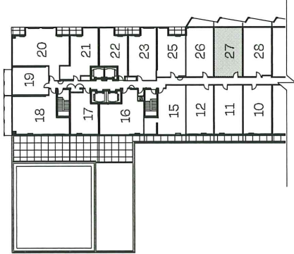
LEVEL 02
