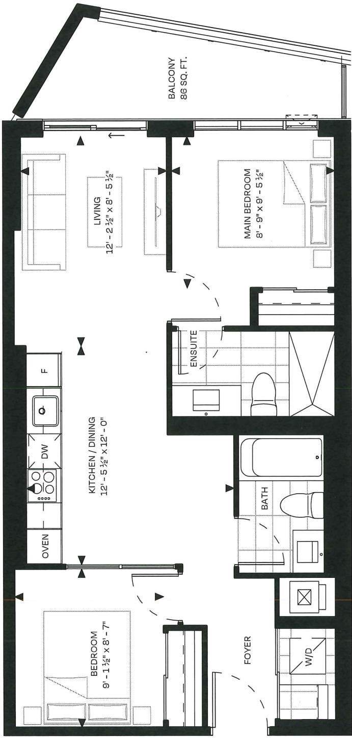
BALCONY AT LEVEL 02 BALCONY DESIGN DIFFERS ON LEVEL 03 & 04
